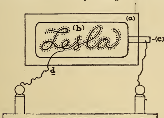
FIG. 95.—Illuminated Sign, Formed by the Effluve Given off from the Fine Wire ( d ) Arranged to Form the Word ( b ), Adhering to the Shellacked Surface of the Glass Plate ( a ). A Sheet of Tin-foil Covers the Back of the Glass and is Connected to a Tesla Terminal by Means of the Copper Strip ( c ), the Opposite Terminal Being Connected to the "Wire Word," ( b ).
