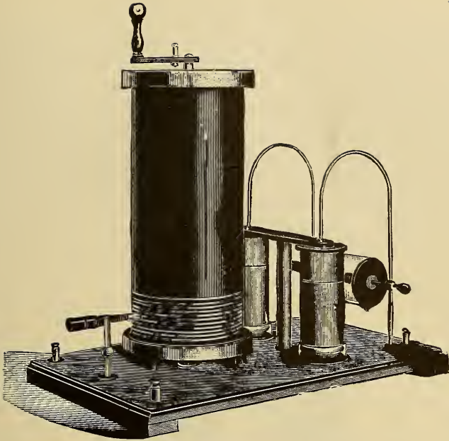
FIG. 9.—Oudin Resonator. (Williams.)
