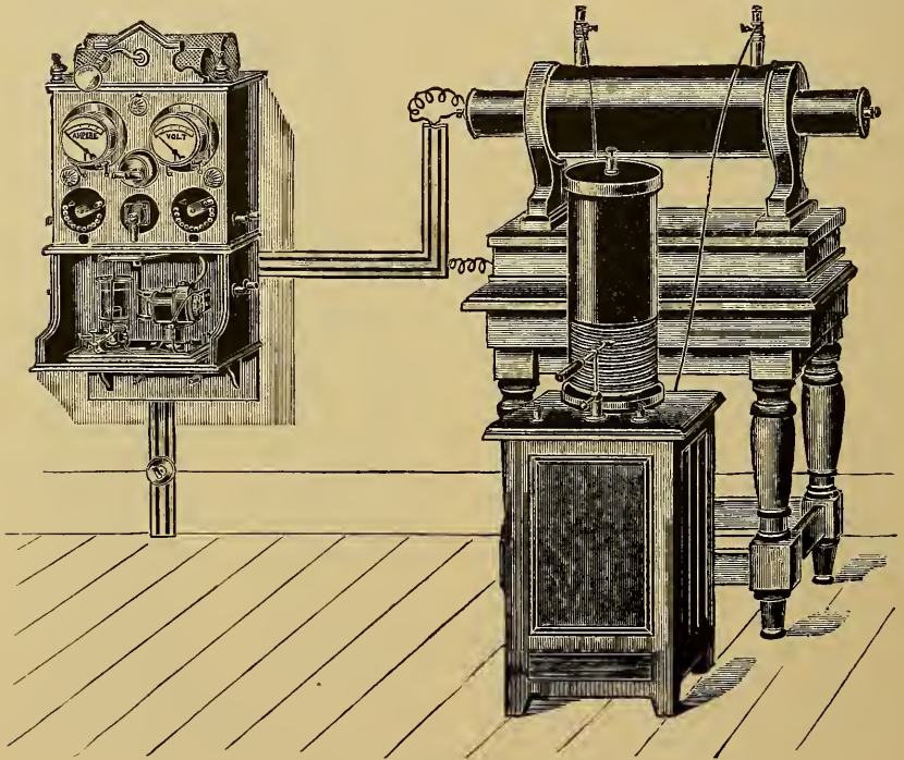
FIG. 42.—Upright Solenoid on Cabinet. (Williams.)
