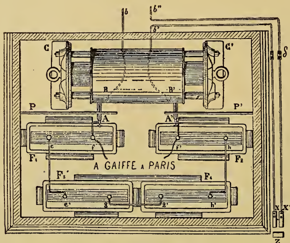
FIG. 51.—Top Shelf of Cabinet. (From Belot.)
