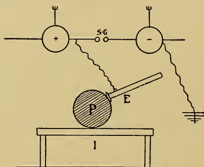
FIG. 157.—Diagram of Static Wave Current.
