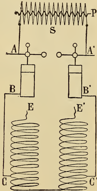
FIG. 41.—Rochefort's Bipolar Resonator. (Freund.)
