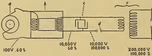
FIG. 62.—Tesla-Thomson High-frequency Apparatus.
