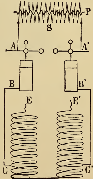
FIG. 11.—Rochefort's Bipolar Resonator. (Guilleminot.)
