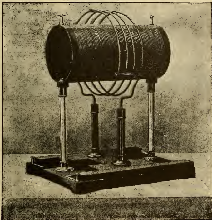
FIG. 7.—D'Arsonval Bipolar High-tension Coil. (Williams.)
