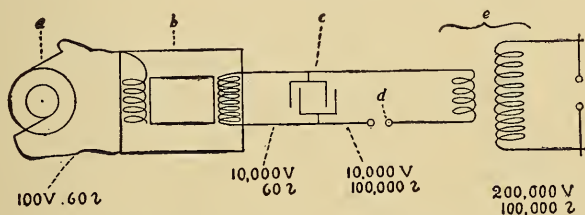
FIG. 89.—Arrangement for the Production of Tesla-Thomson Currents.
