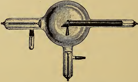
FIG. 139.—X-Ray Tube with Solid Metal Anode.
