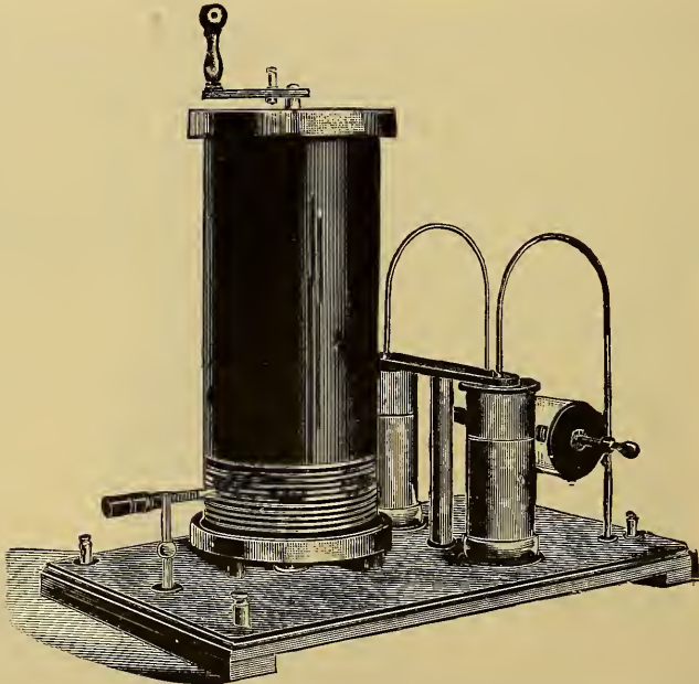
FIG. 56.—Resonator and Condensers (small model). (Williams.)
