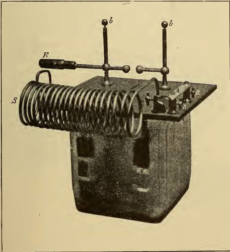
FIG. 44.—Gaiffe's Oil Condenser and Heavy Solenoid.
