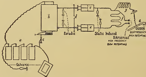
FIG. 88.—Arrangement for the Production of Oudin-d'Arsonval Currents.
