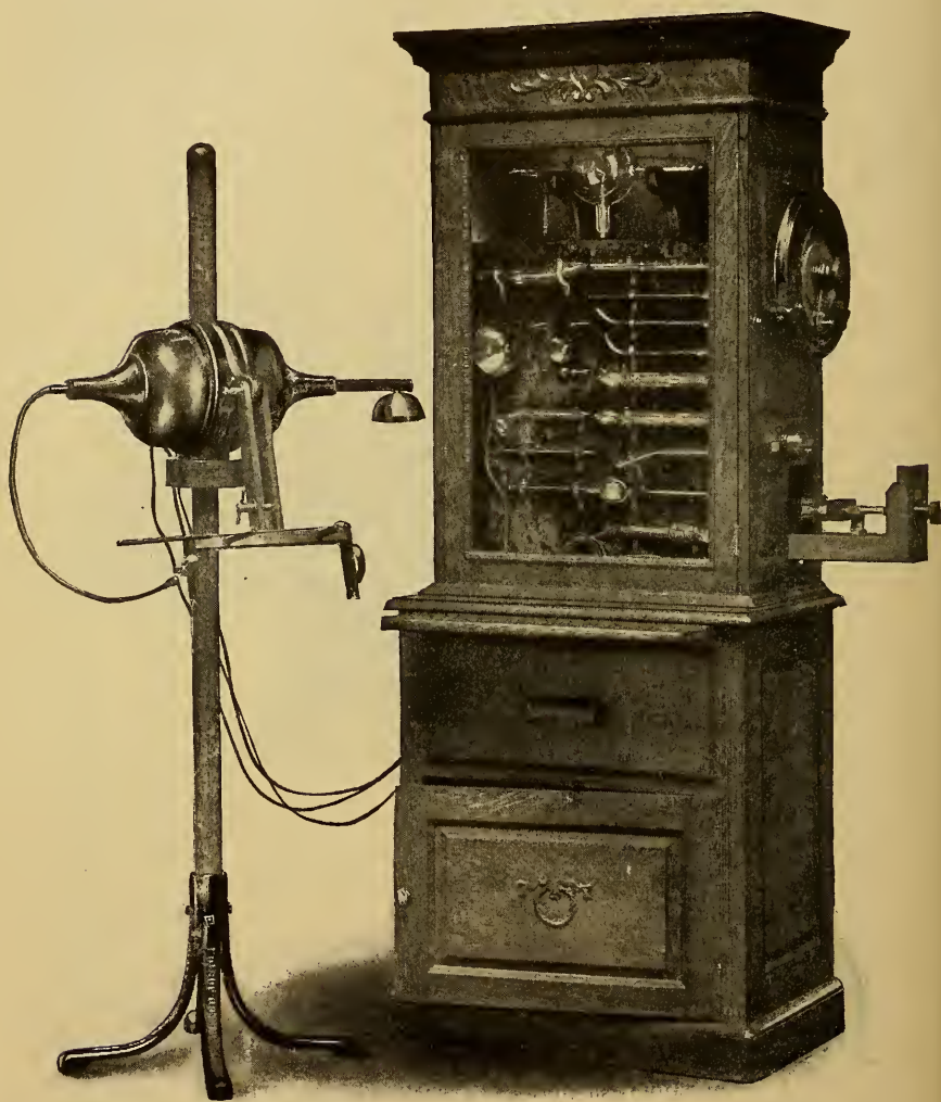
FIG. 71.—Jackson Coil with Separate Secondaries.
