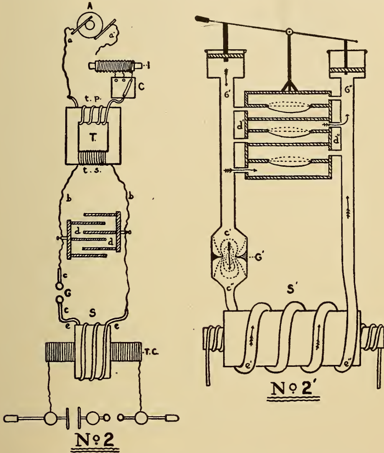
FIG. 27.—Plate II. Tesla-Thomson Circuit and Hydraulic Analogue.
