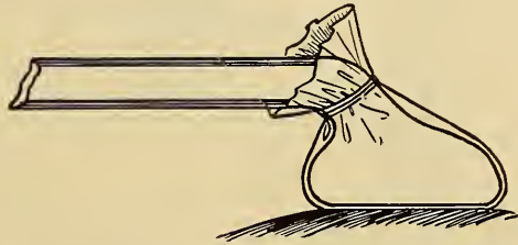
FIG. 162.—Vacuum Electrode Covered with Chamois Skin.
