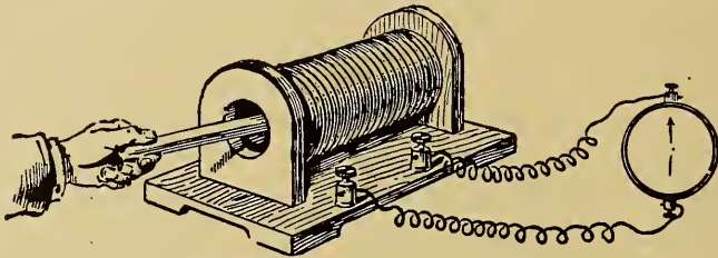
FIG. 21.—Magnetic-electric Induction. (Williams.)
