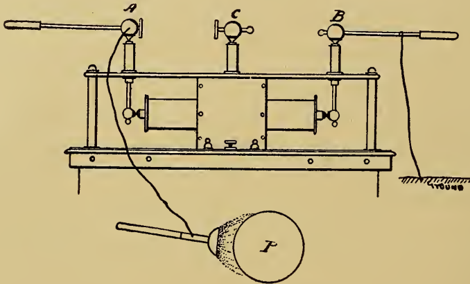
FIG. 13.—The Author's Air-gap Condenser Terminals.
