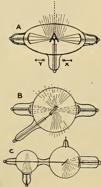
FIG. 143.—Types of "High-frequency X-Ray Tubes." A, Thomson Double Focus. B, Strong Double Focus. C, Single Focus (double bulb).
