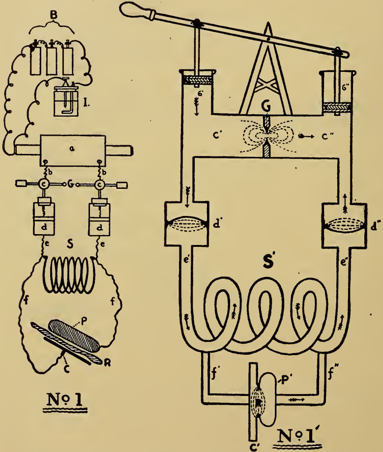
FIG. 27.—Plate I. D'Arsonval Circuit and Hydraulic Analogue.
