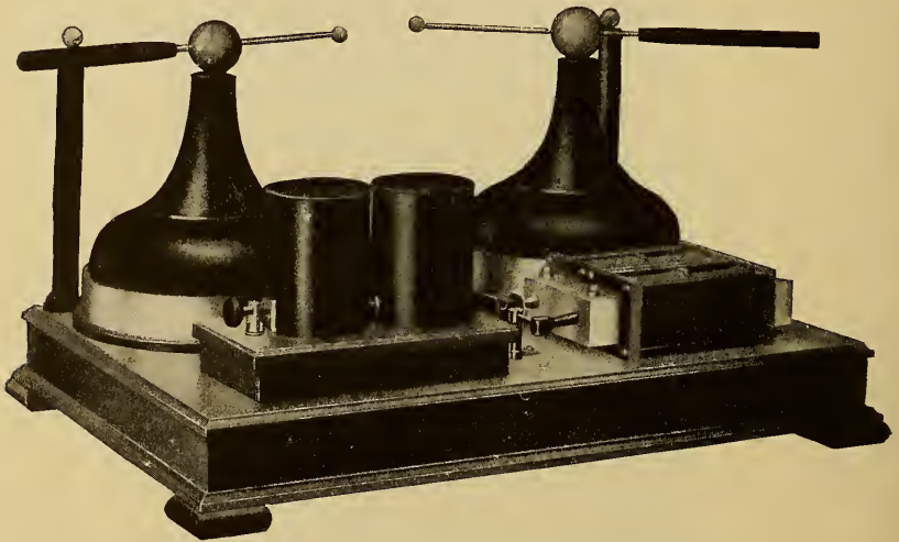
FIG. 66.—Kinraide Coil with Improved Spark-gap.
