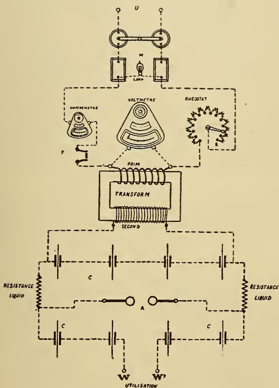
Fig. 50.—General Diagram. (From Belot.)
