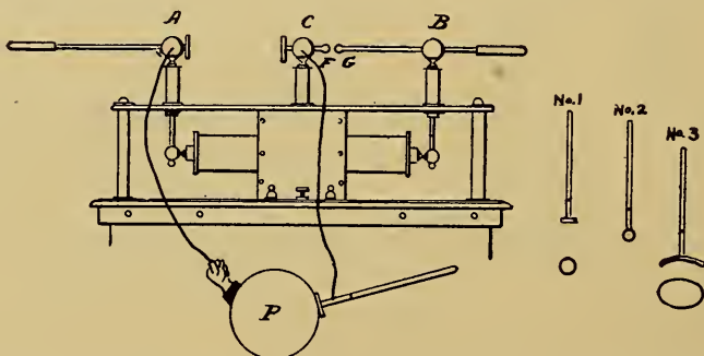
FIG. 121.—High-frequency Motor-impulse Current. ("Pseudo-faradic.")
