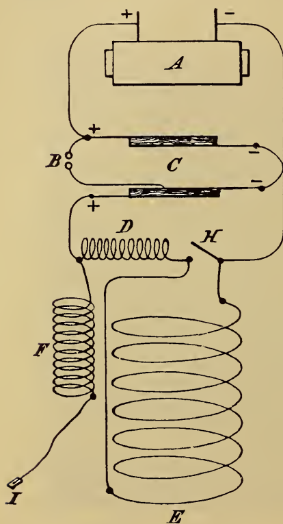
FIG. 8.—Diagram of Solenoid and Resonator. (Freund.)
