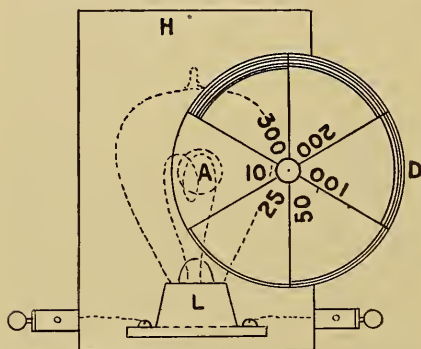
FIG. 106.—The Author's Photometric Mil-ammeter.
