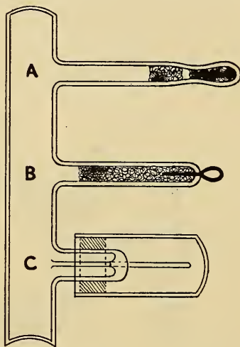
FIG. 141.—Vacuum Regulators for X-Ray Tubes.
