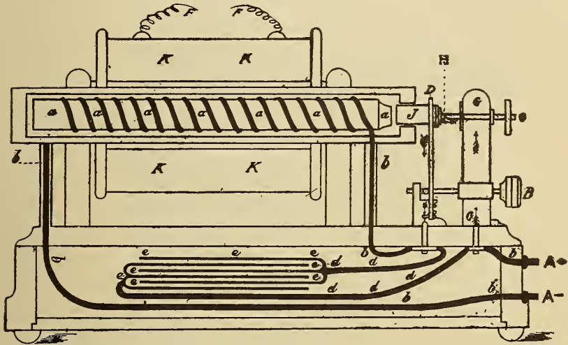
FIG. 34.—Ruhmkorff Induction Coil, Shown Diagrammatically. (Williams.)
