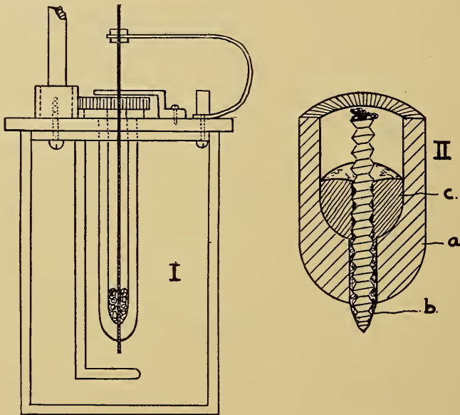
FIG. 85.—The Author's Improved Electrolytic Interrupter.
