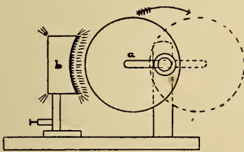
FIG. 120.—The Author's Mechanism for Superimposing a Low Frequency, Sinusoidal Wave Upon a Tesla Current.
