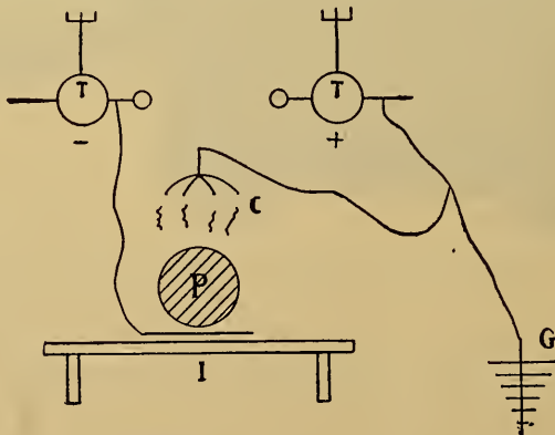
FIG. 154.—“Static Breeze.” (Diagram.)
