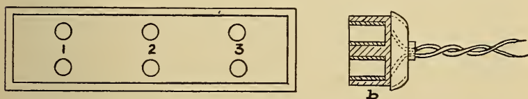
Fig. 74.—“Theater Plug,” for varying current strength on “Cyclone” and “Ajax Special Coils.”
