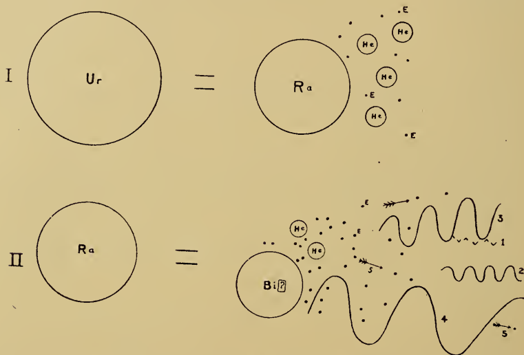
FIG. 15.—Schematic Diagram Showing Spontaneous Degeneration of Atoms.
