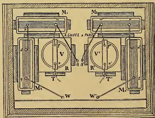
FIG. 52.—Lower Shelf of Cabinet. (From Belot.)
