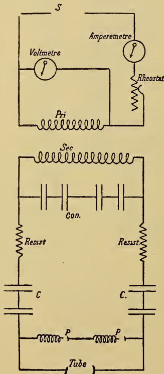
FIG. 54.—Regulating Apparatus. Arrangement of Transformer. (From Belot.)
