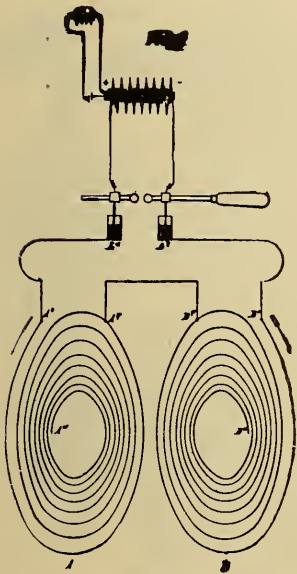
FIG. 40.—Resonator of Lebailly and O'Farril.
