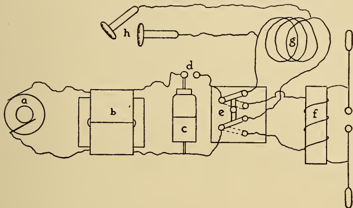
FIG. 59.—Diagram of the Author's Apparatus, Adapted for the Generation of heavy D'Arsonval Currents, as well as those of the High-potential ("Tesla") type.
