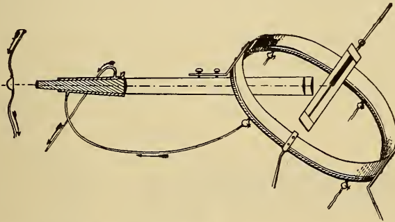
FIG. 148.—Diagram of Finsen's Arc Lamp. (Guilleminot.)
