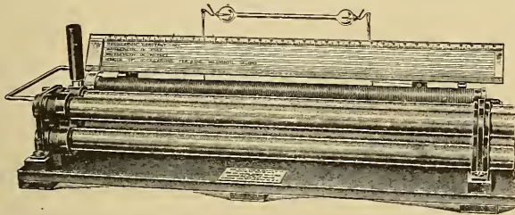
FIG. 107.—Professor Fleming's "Direct-reading Cymometer." (Marconi Wireless Telegraph Co.)
