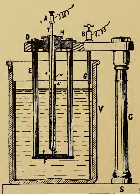
FIG. 31.—Electrolytic Interrupter of Wehnelt. (Williams.)
