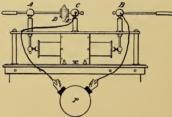
FIG. 119.—High-frequency "Motor-Wave Current."
