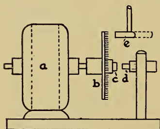
FIG. 77.—The Author's Improved Rotary Spark-gap.
