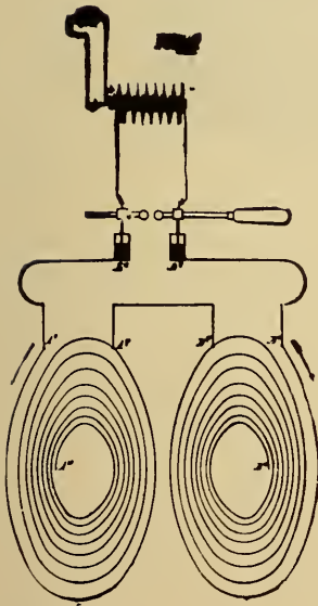
Fig. 10.—Bipolar Resonator of O'Farril.
