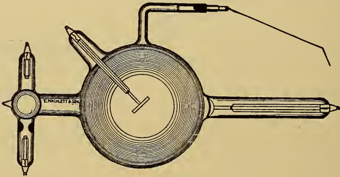
FIG. 142.—"Self-regulating" X-Ray Tube.
