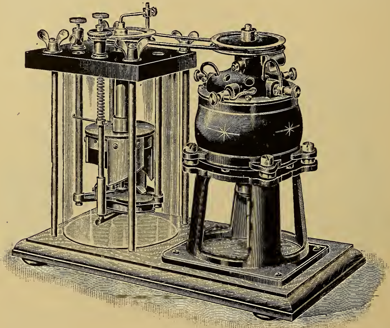
FIG. 35.—Mercury Jet Interrupter. (Isenthal & Co.)
